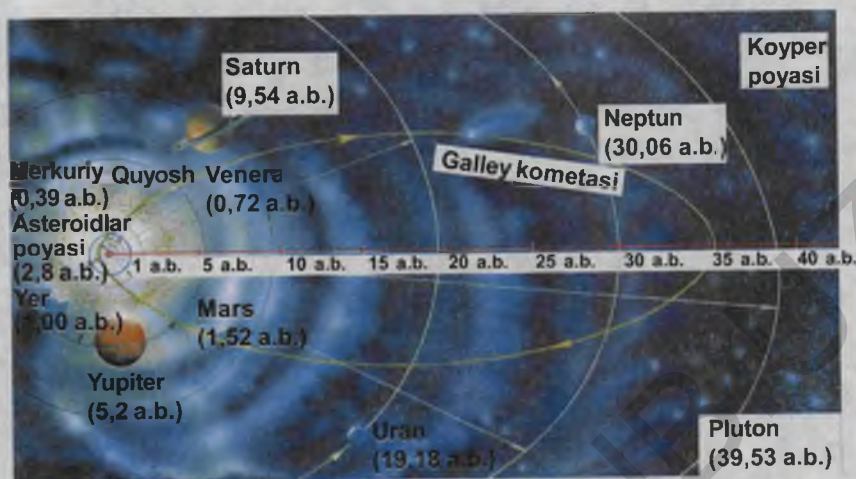
26- rasm. Quyosh sistemasining mashtabi.
