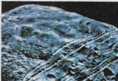
85- rasm. Marsning Fobos deb ataluvchi yo'ldoshi (o'lchami 18×22 km).
