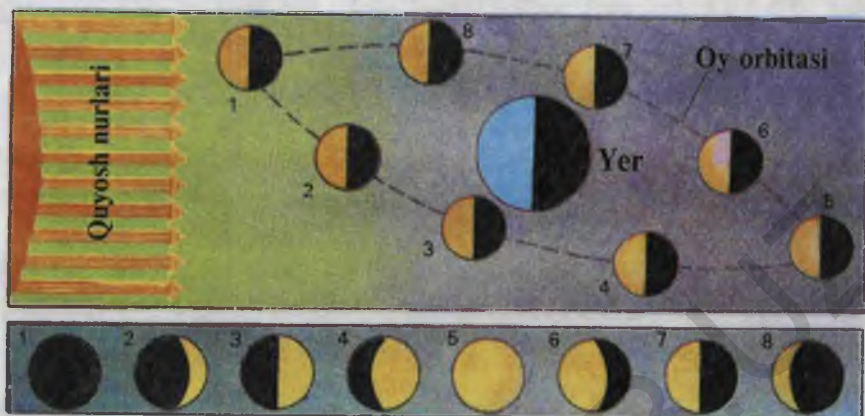
33- rasm. Oy fazalarining almashinishi
